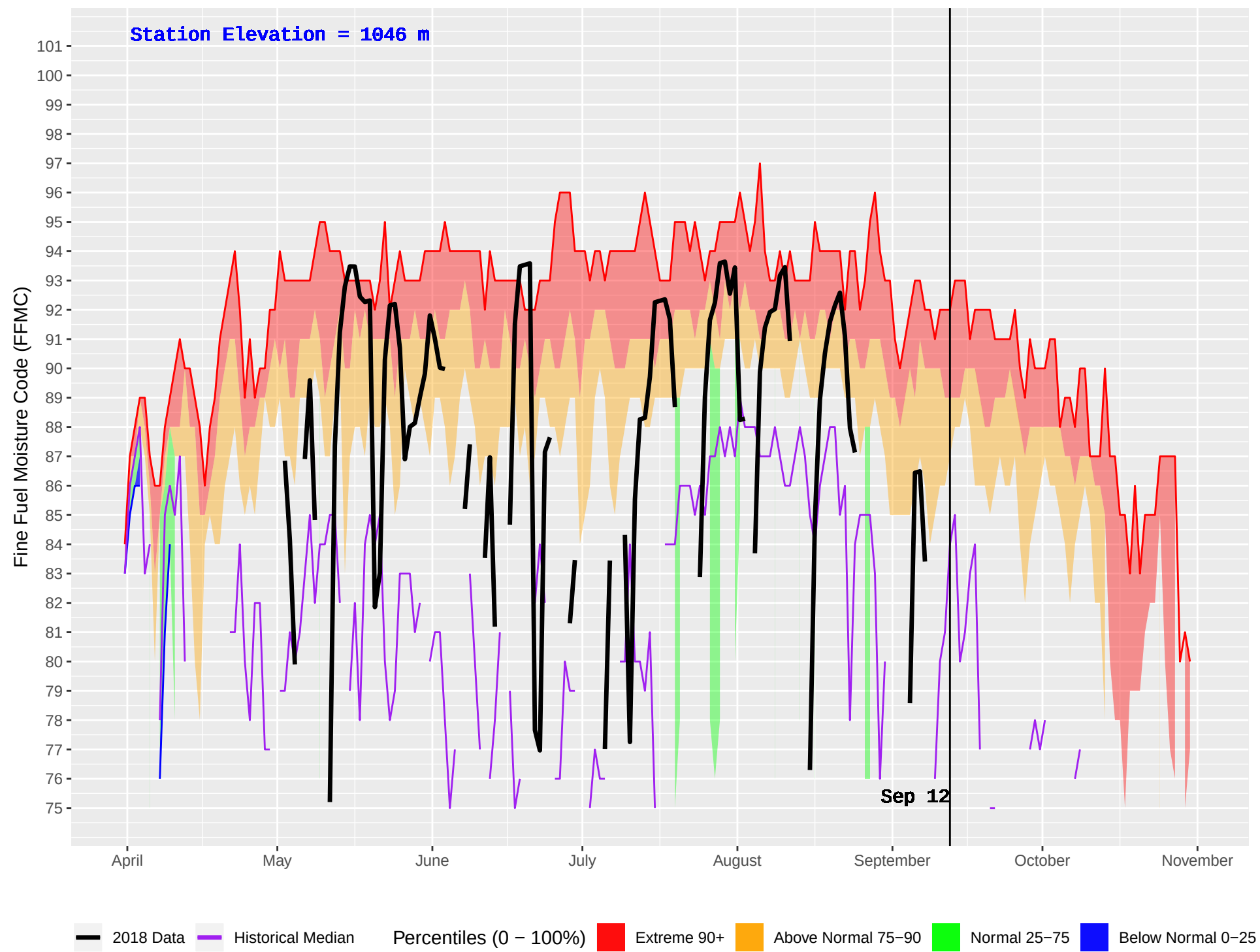
LIKELY RS (255) : Historical (1970–2016) and Current (2018) Daily Fine Fuel Moisture Code (FFMC)
