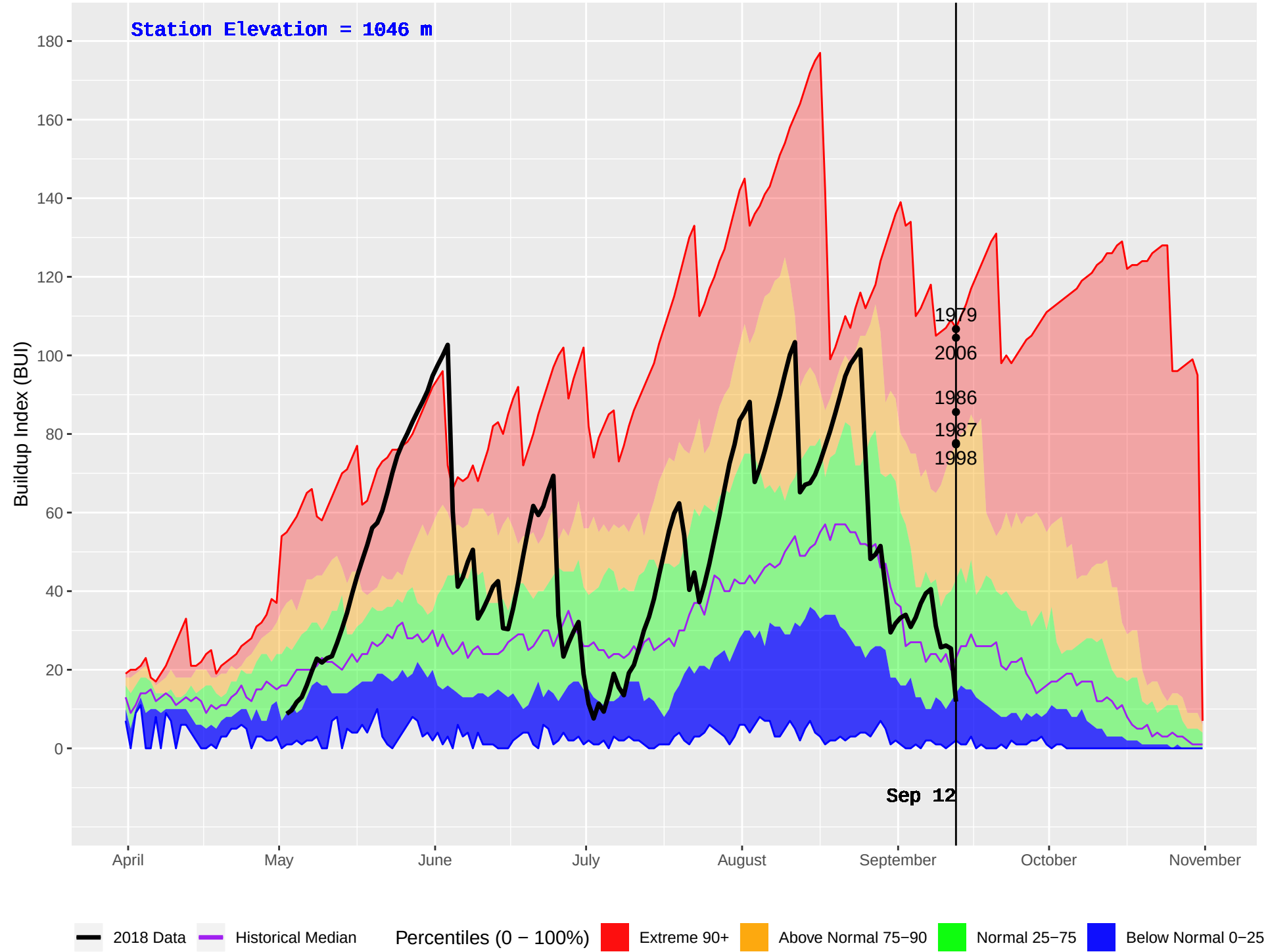
LIKELY RS (255) : Historical (1970–2016) and Current (2018) Daily Buildup Index (BUI)
