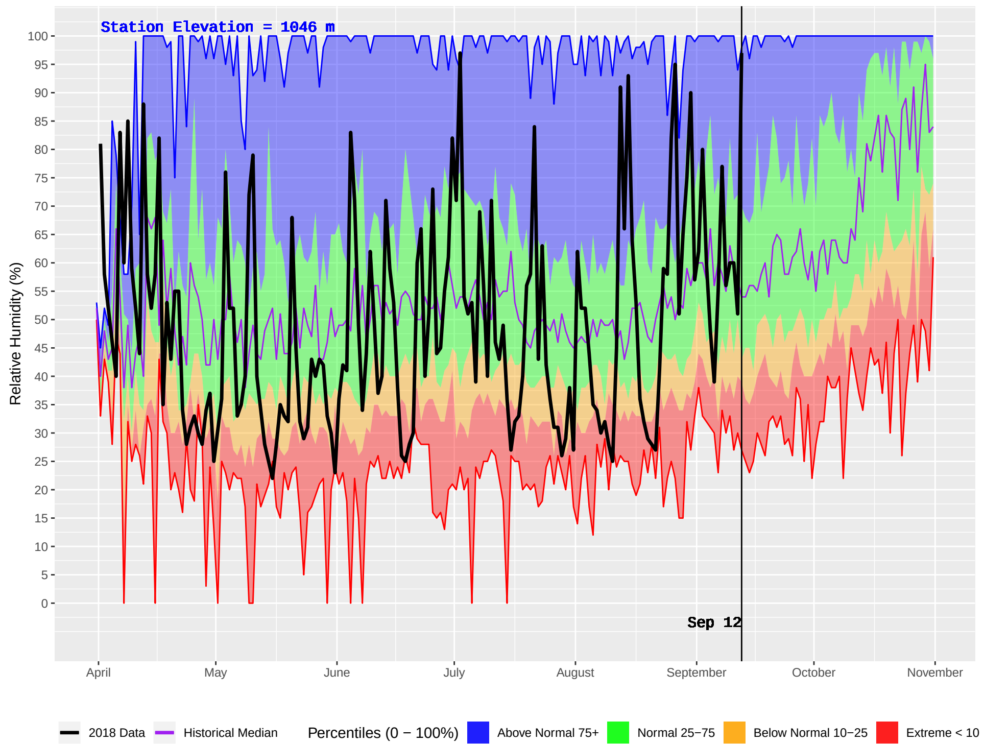
LIKELY RS (255) : Historical (1970–2016) and Current (2018) Daily Relative Humidity
