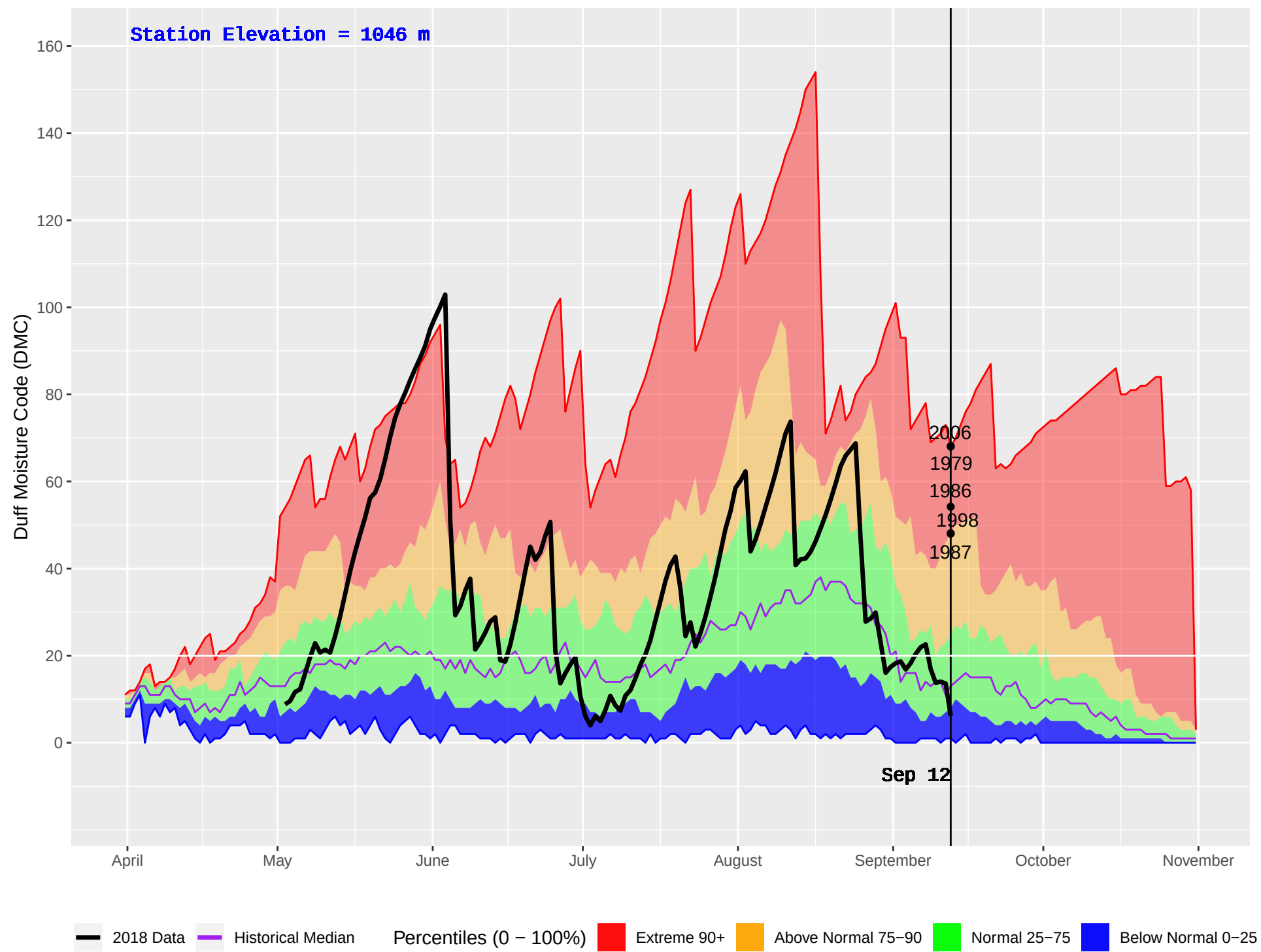
LIKELY RS (255) : Historical (1970–2016) and Current (2018) Daily Duff Moisture Code (DMC)
