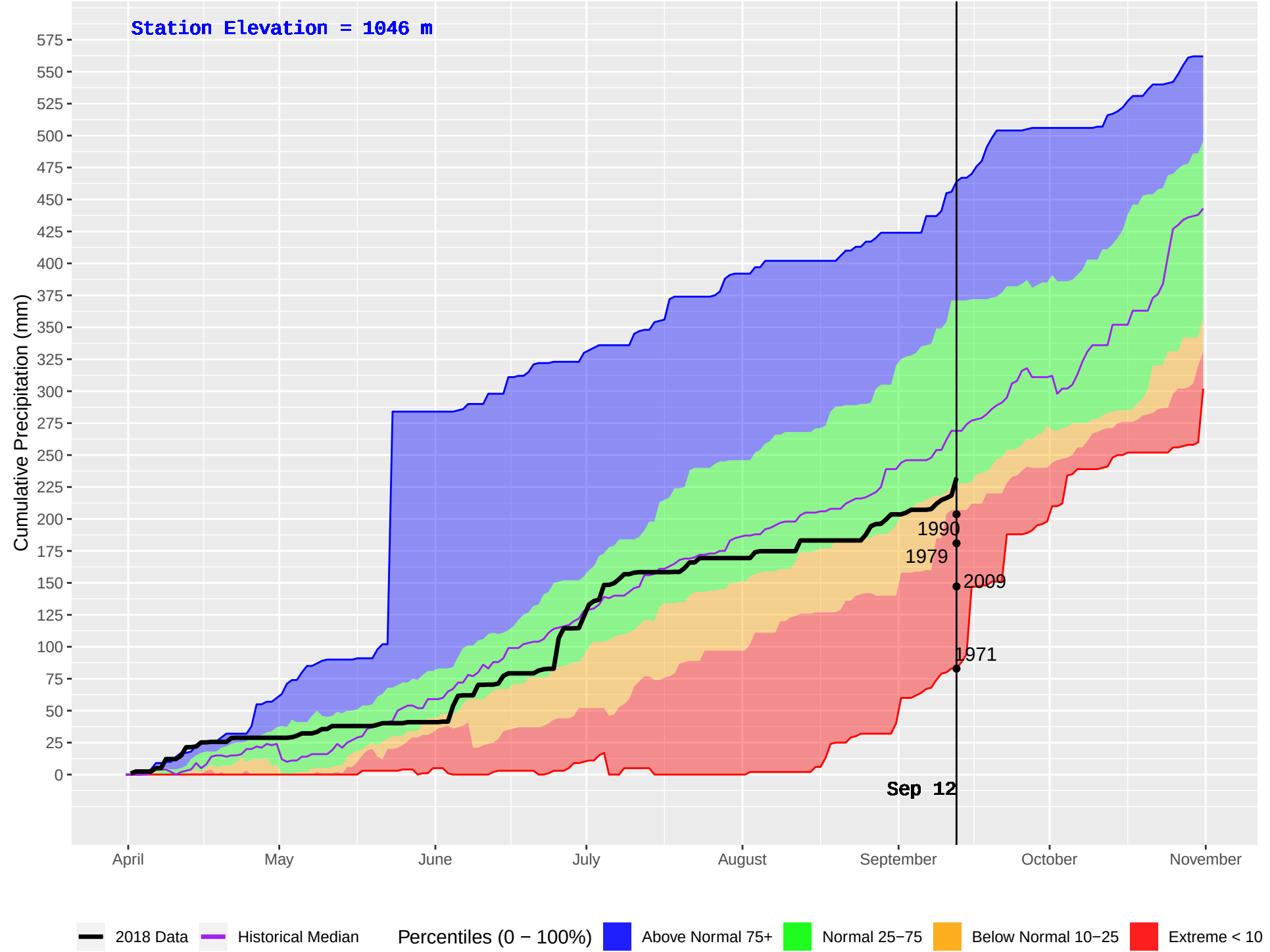
LIKELY RS (255) : Historical (1970–2016) and Current (2018) Daily Cumulative Precipitation
